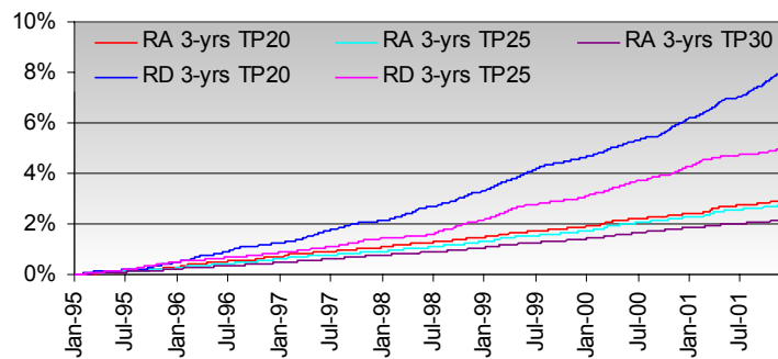
Figure 7 Cumulative transaction costs for different tracking portfolios and stock selection methods
