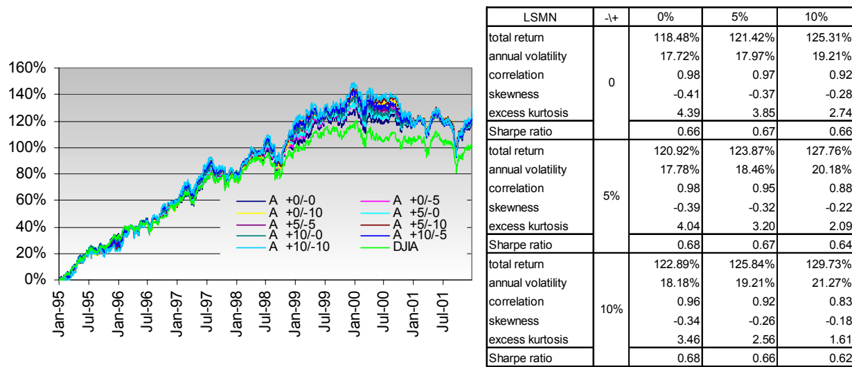
Figure 18 Cumulative returns on the alpha transport strategy
