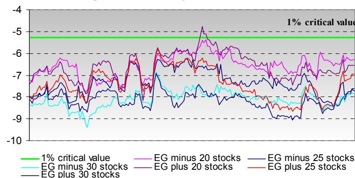
Figure 9 ADF test statistics for portfolios tracking \pm 15\% benchmarks (calibration period 5 years)
